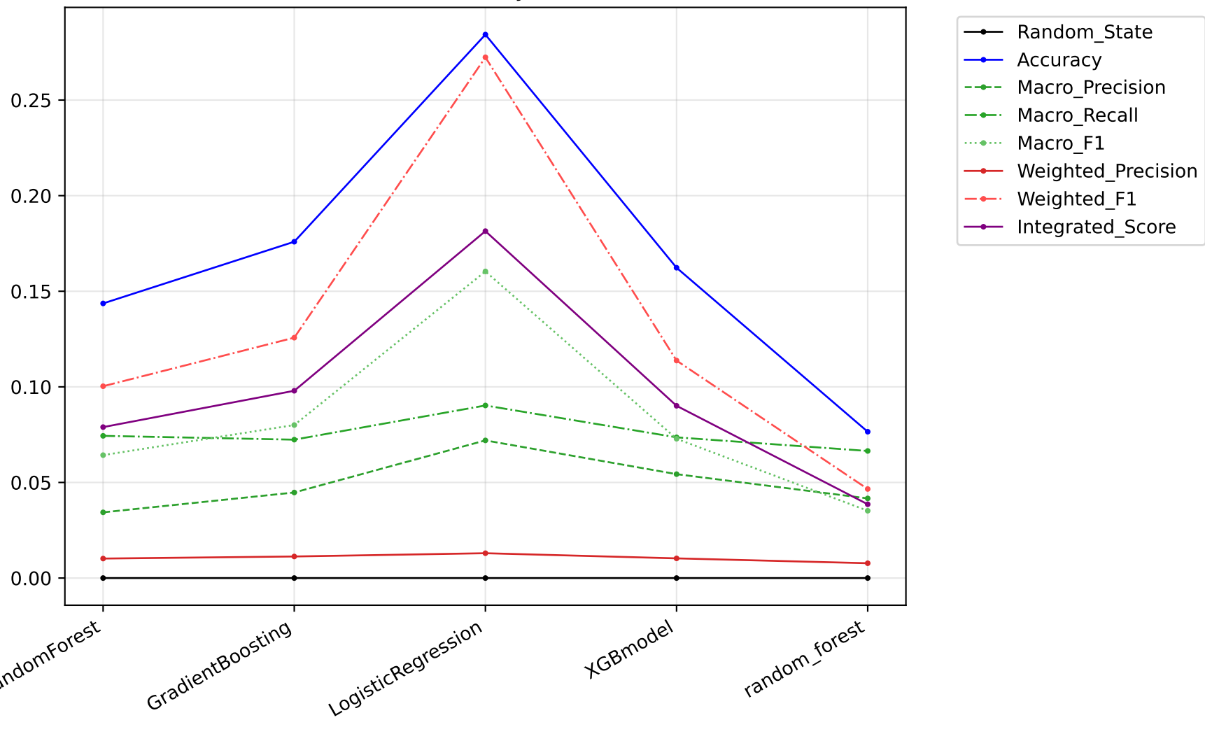
Std Metrics by Model
