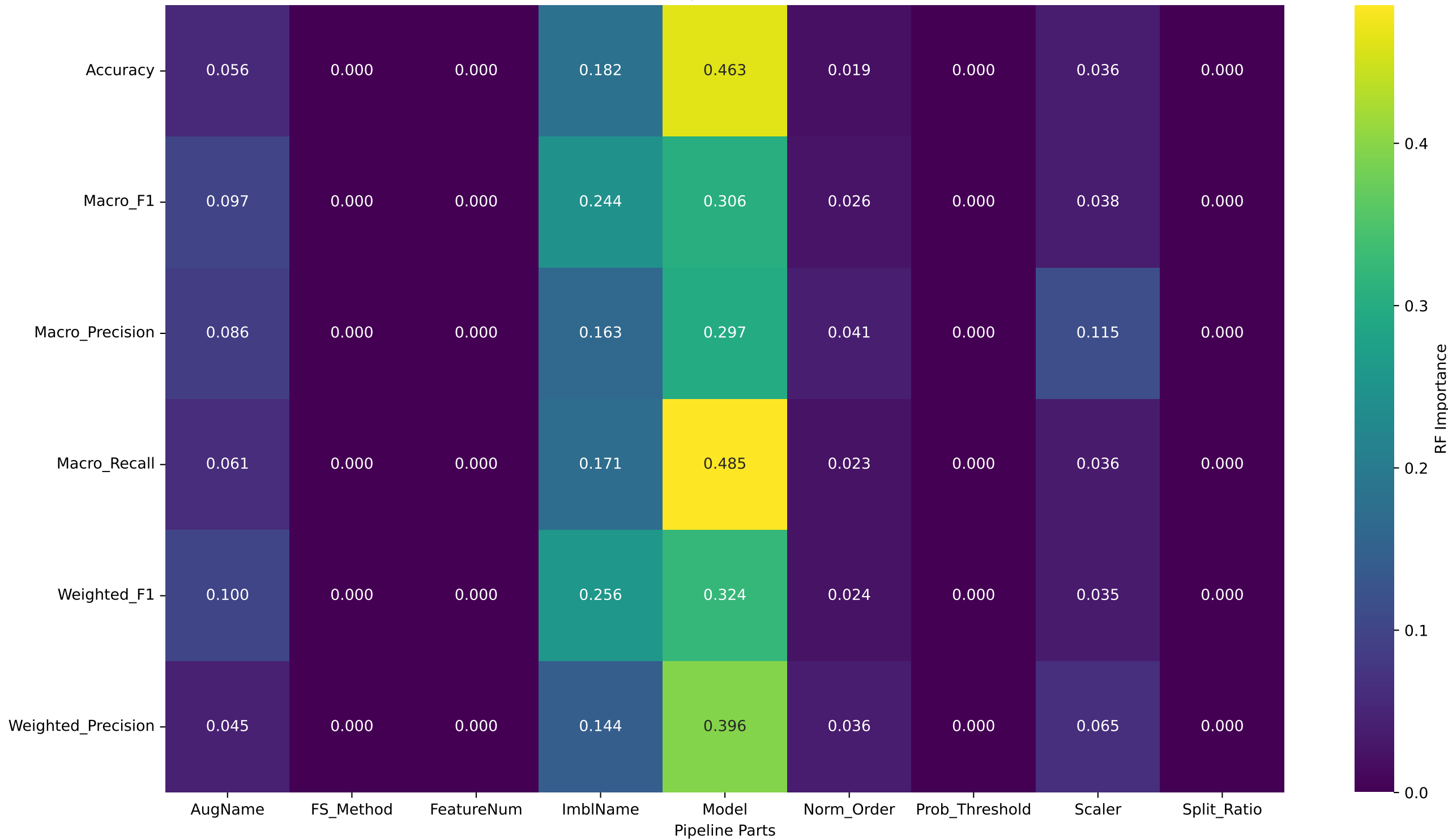
Random Forest Importance: Parts vs Metrics
