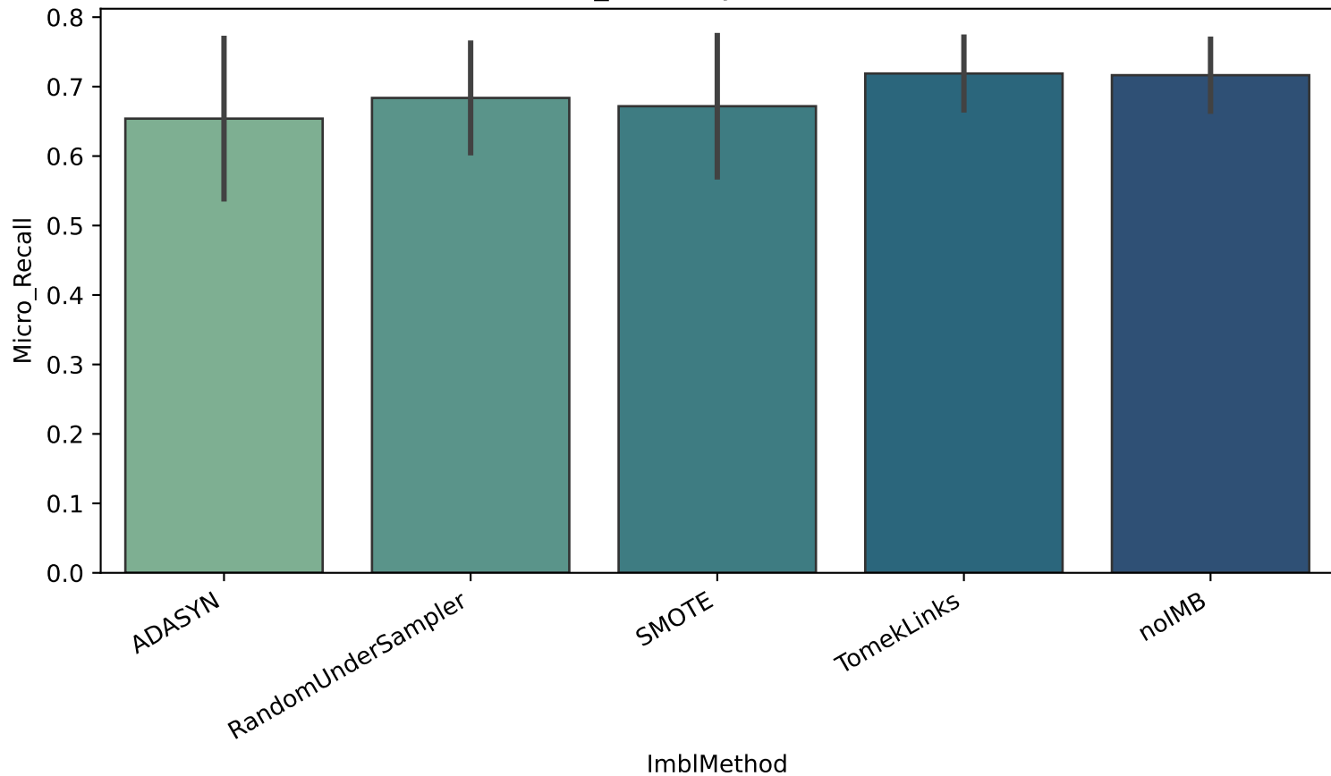
Micro_Recall by ImblMethod
