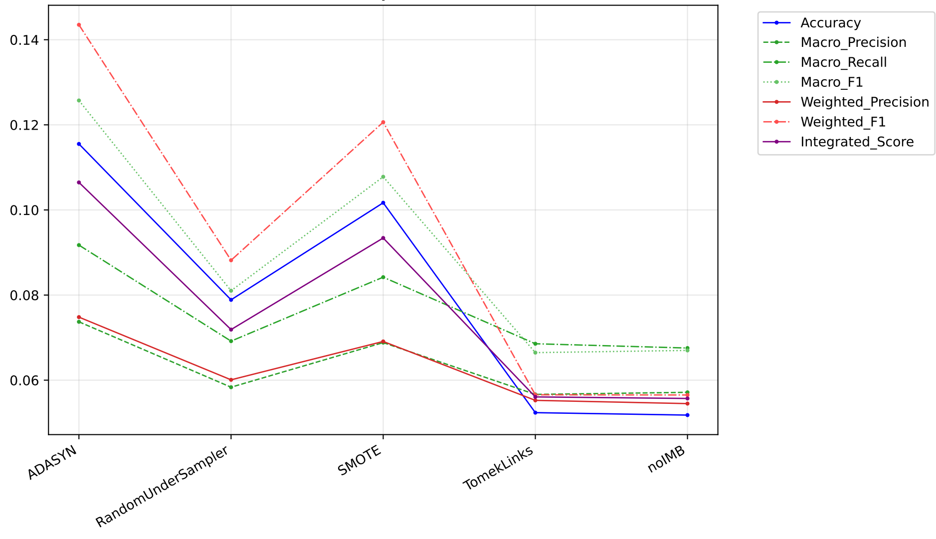
Std Metrics by ImblMethod
