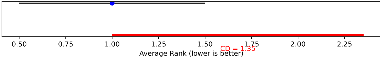
random_forest CD Diagram (Micro_F1)
