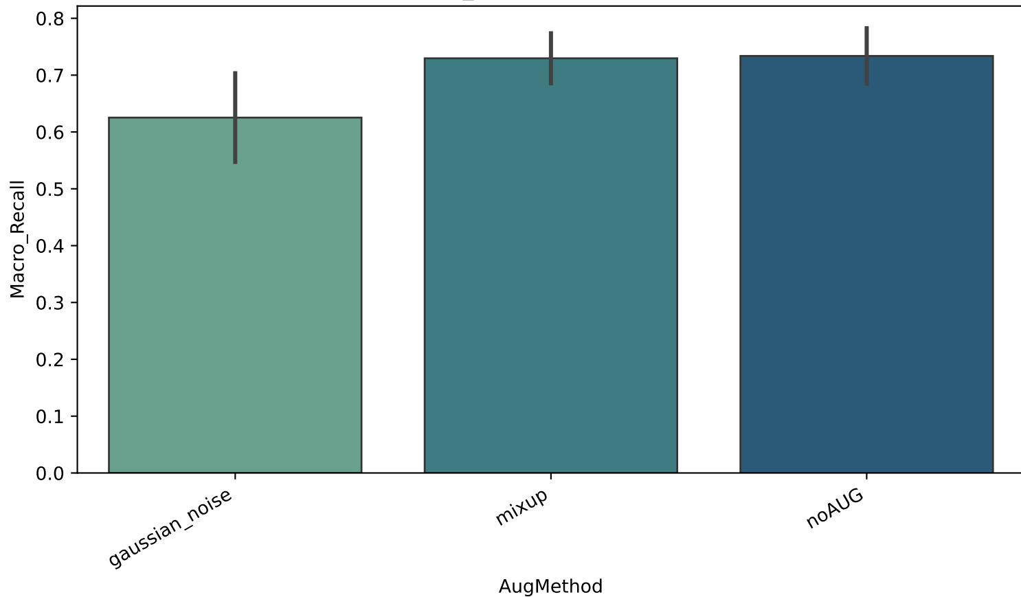
Macro_Recall by AugMethod
