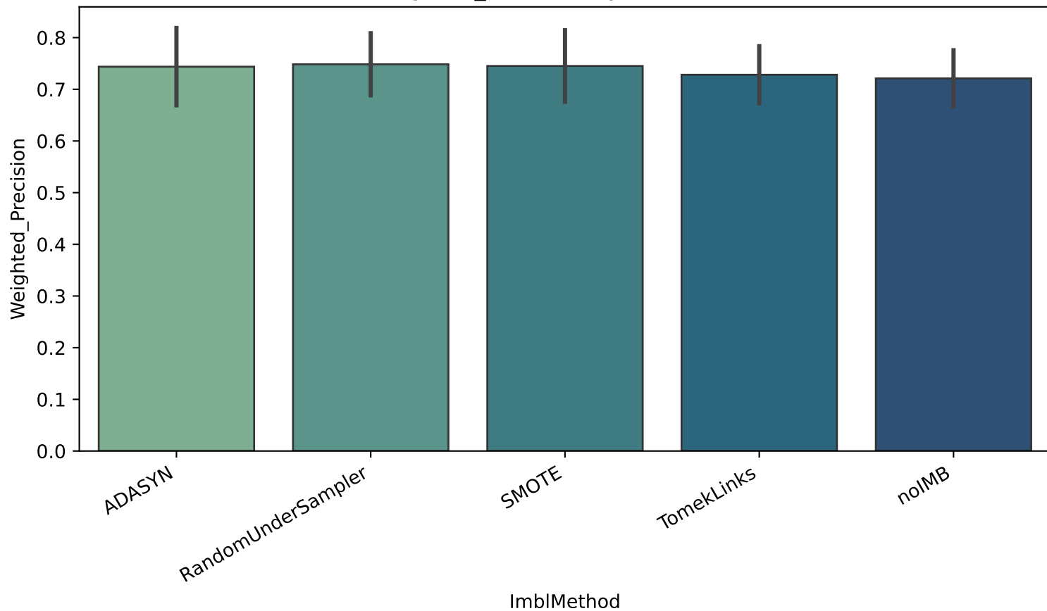
Weighted_Precision by ImblMethod
