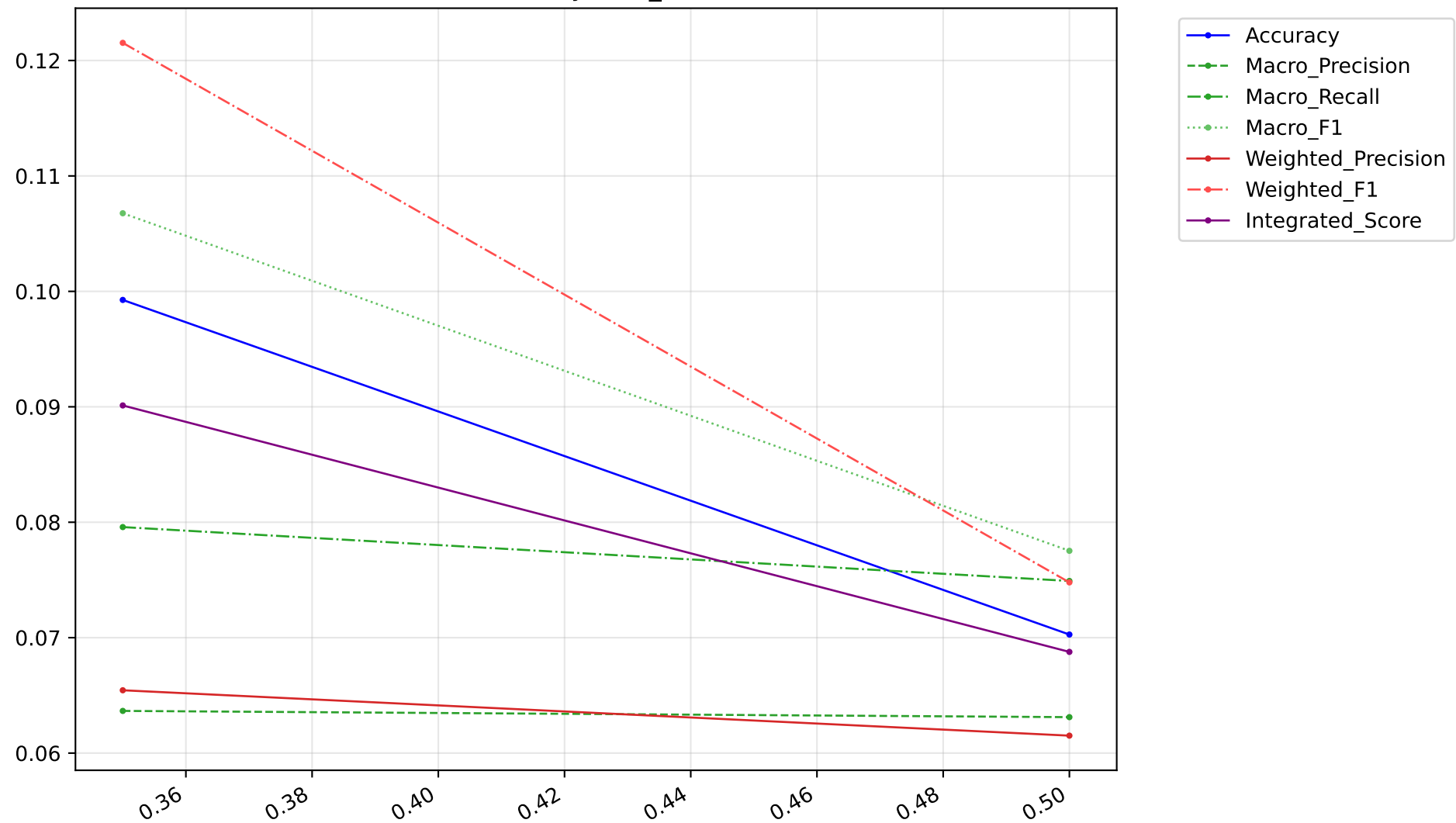
Std Metrics by Prob_Threshold
