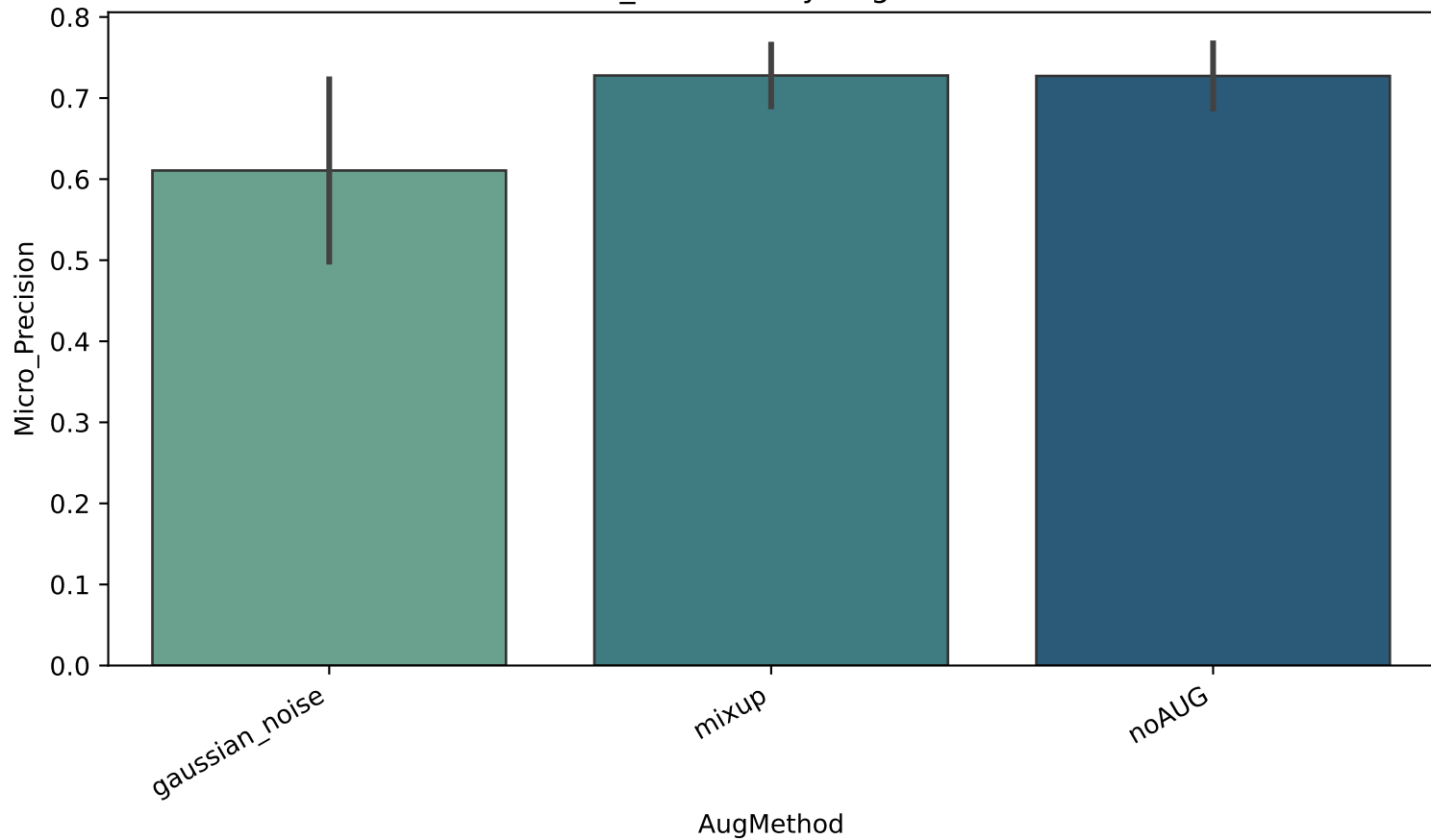
Micro_Precision by AugMethod
