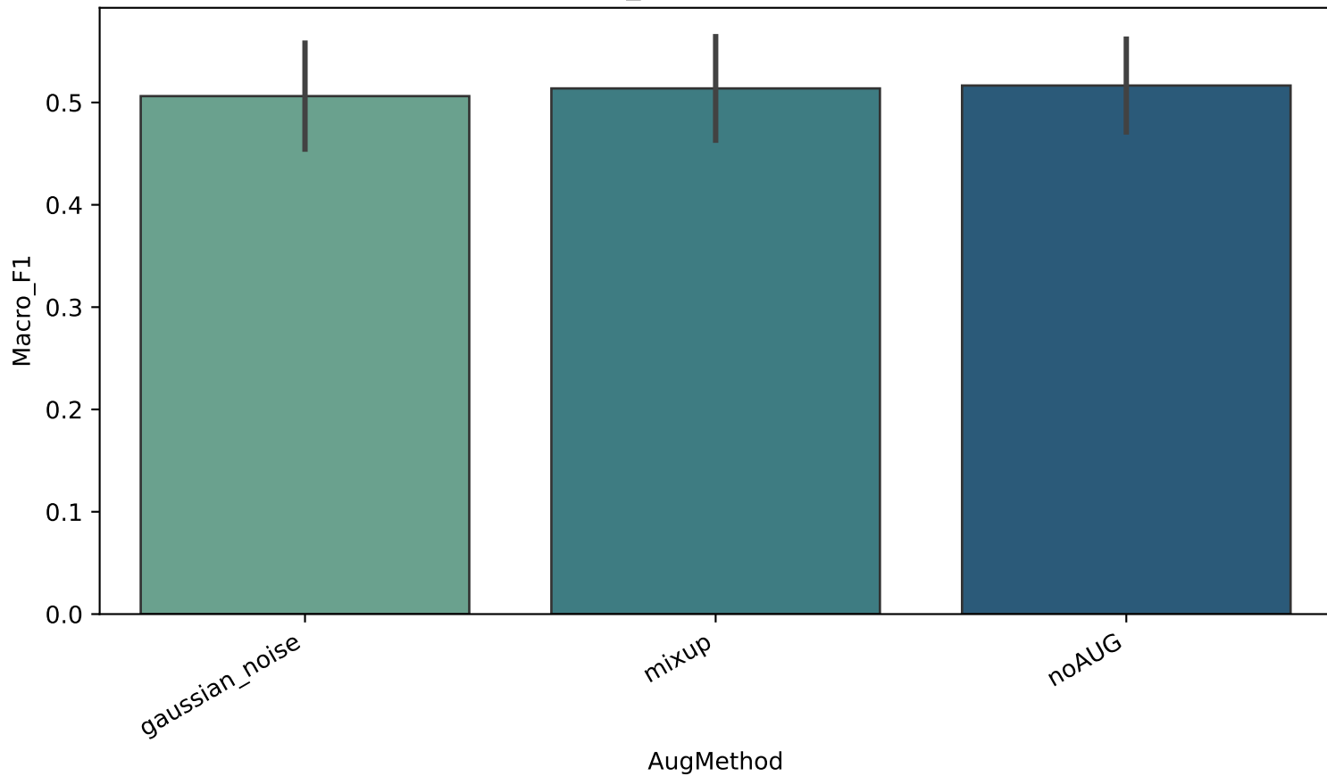
Macro_F1 by AugMethod
