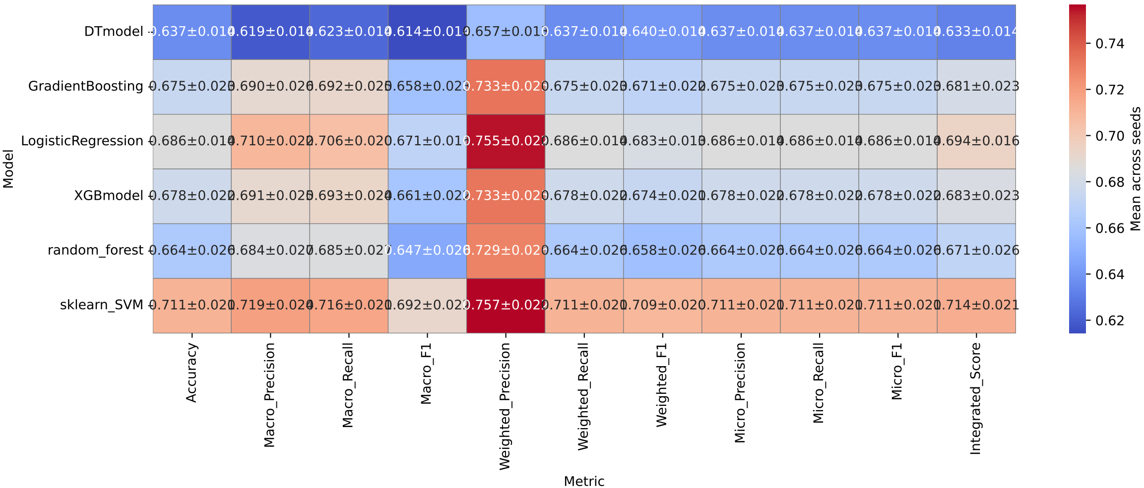
Cross-Seed Performance Deviation (mean \pm std)
