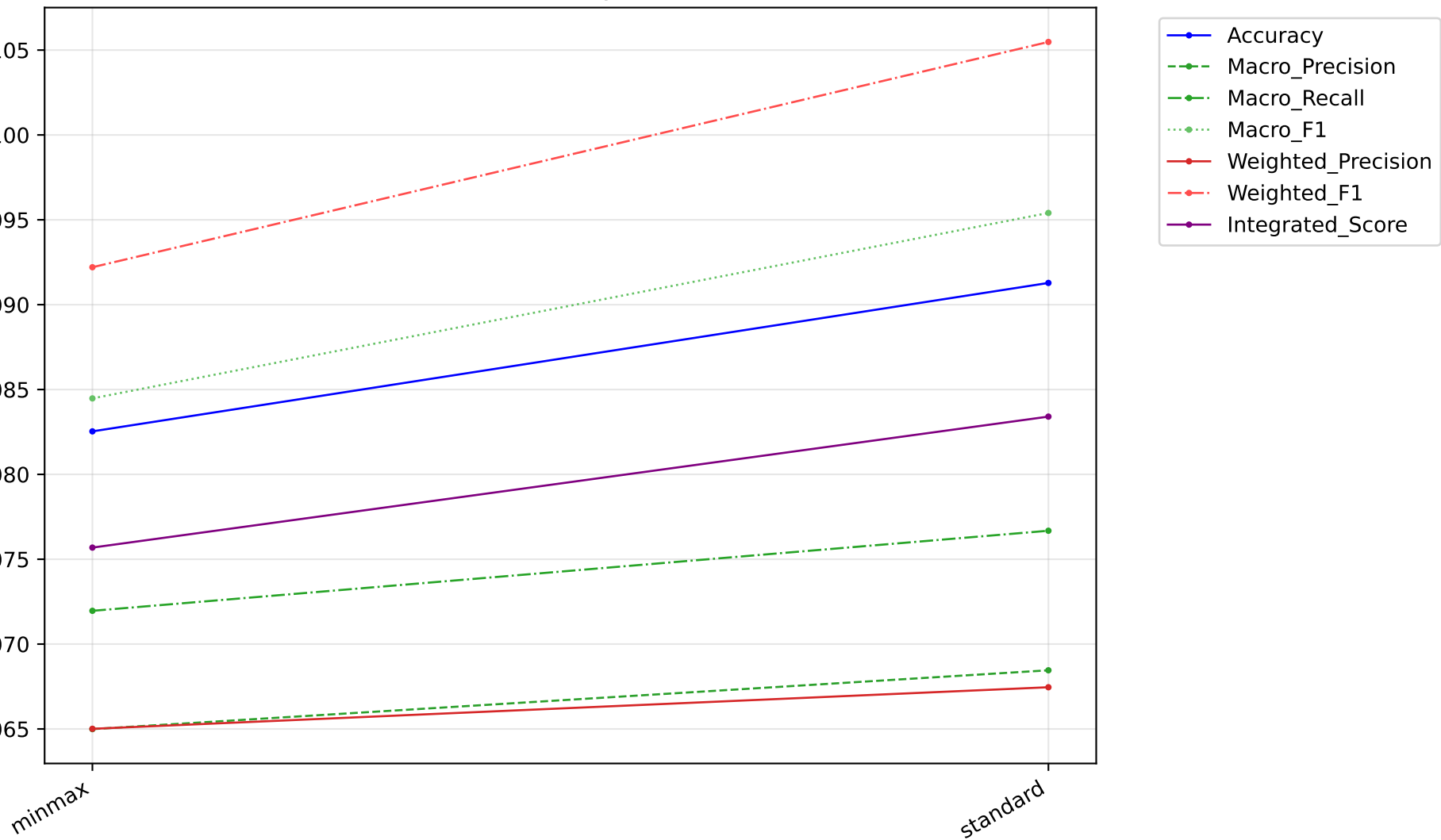
Std Metrics by Scaler
