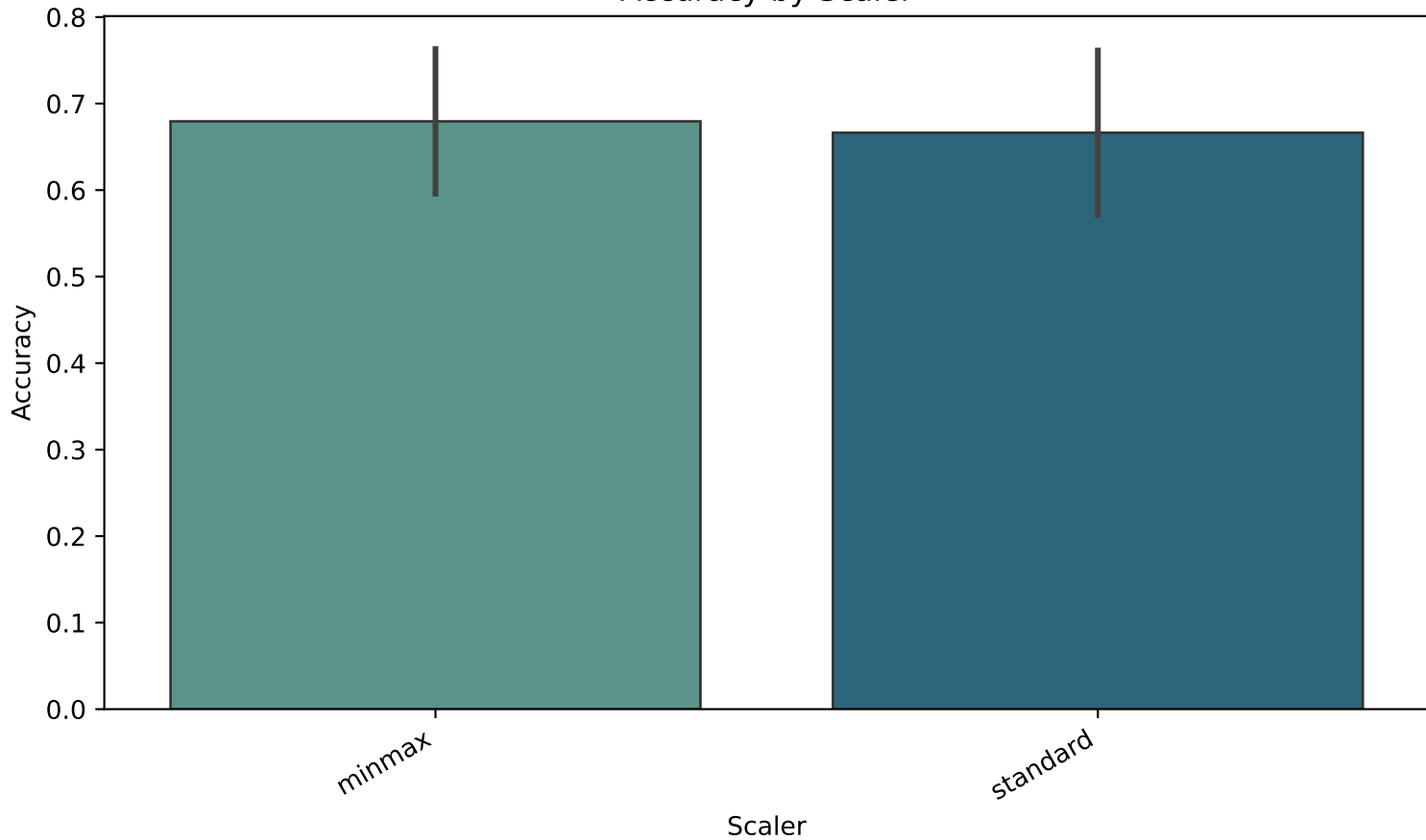
Accuracy by Scaler
