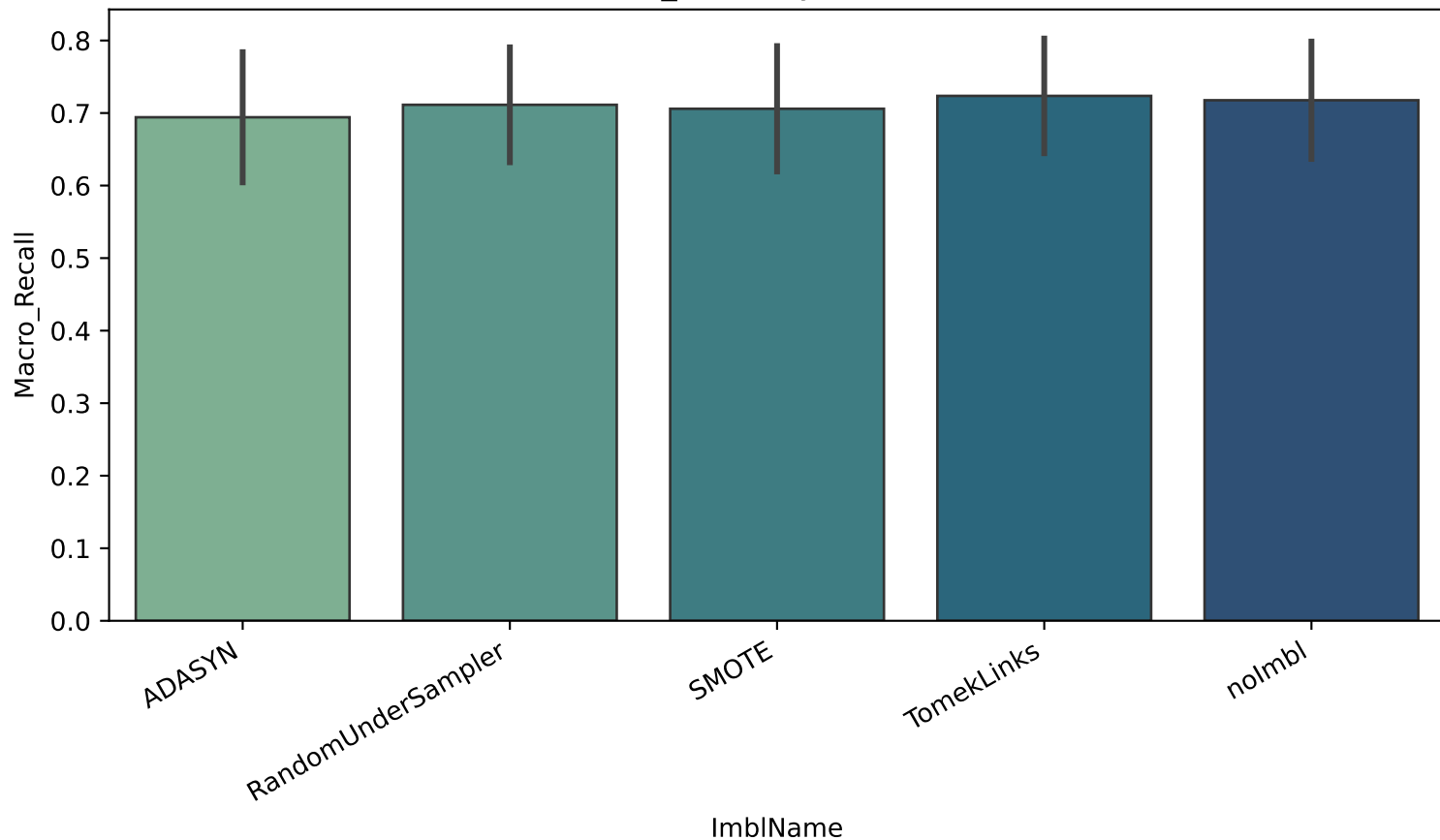
Macro_Recall by ImblName
