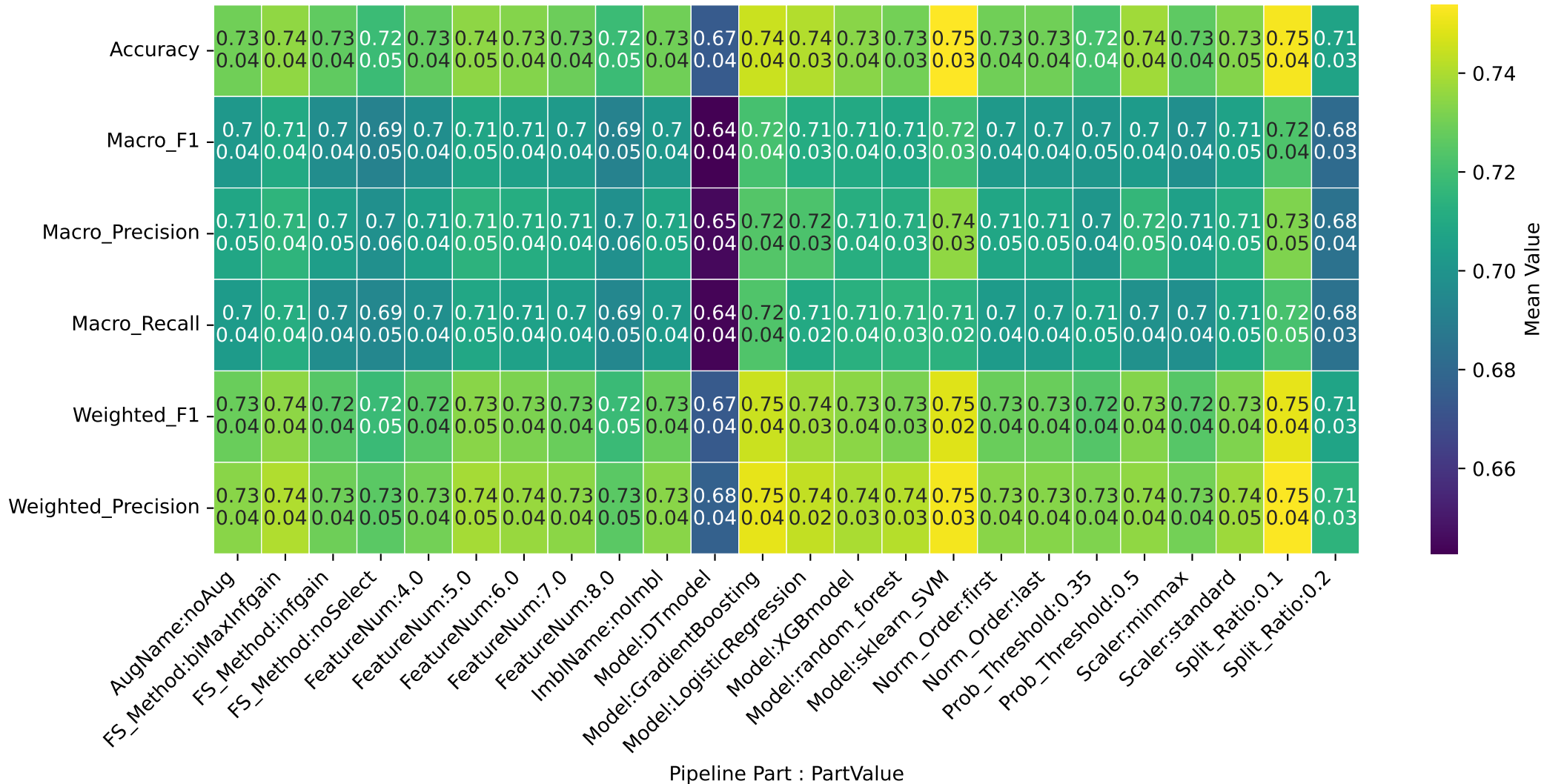
Pipeline Metrics Heatmap (Mean ± Std)
