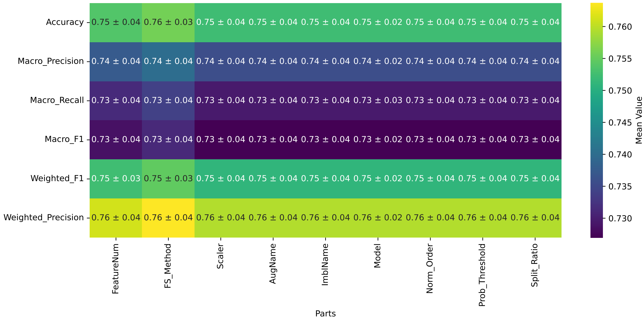
Metrics vs Parts (Mean ± Std)
