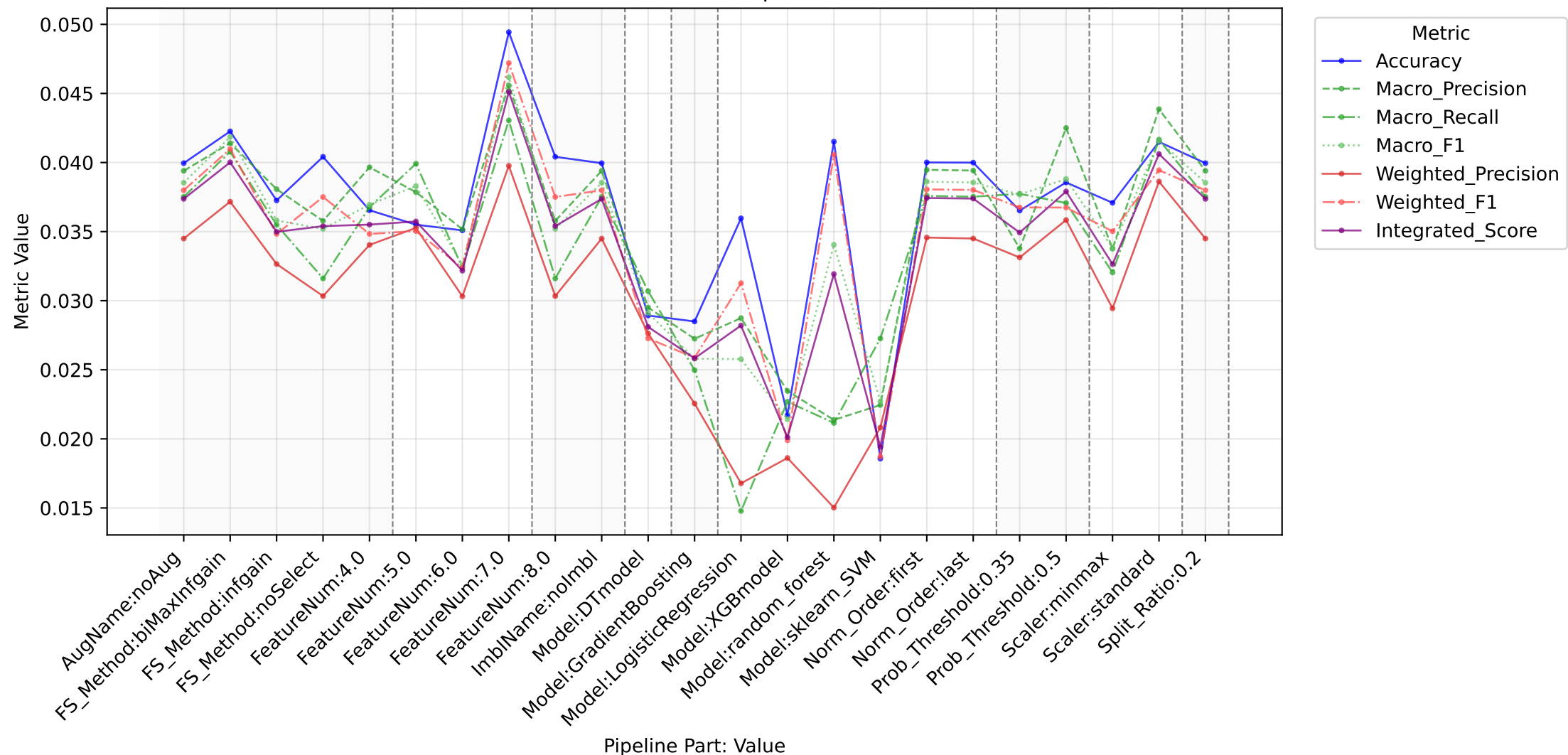
All std Metrics Across Pipeline Parts
