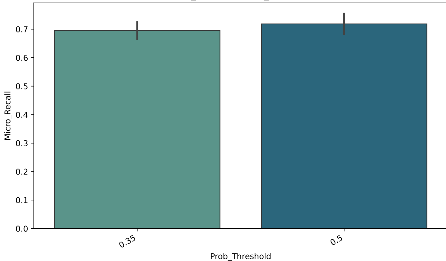
Micro_Recall by Prob_Threshold
