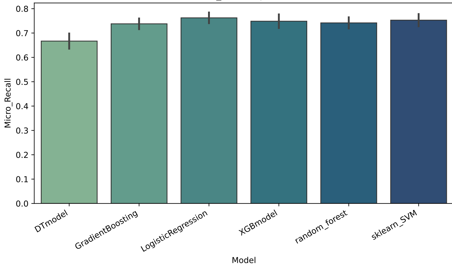
Micro_Recall by Model
