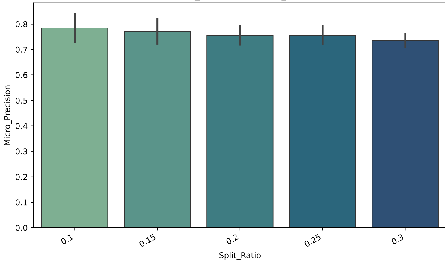
Micro_Precision by Split_Ratio
