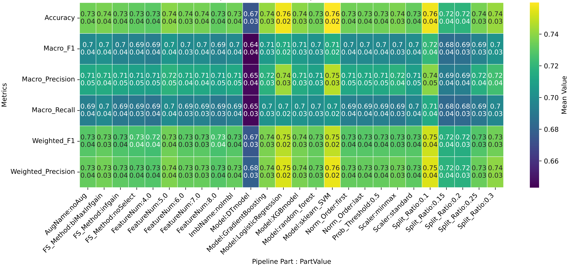
Pipeline Metrics Heatmap (Mean \pm Std)
