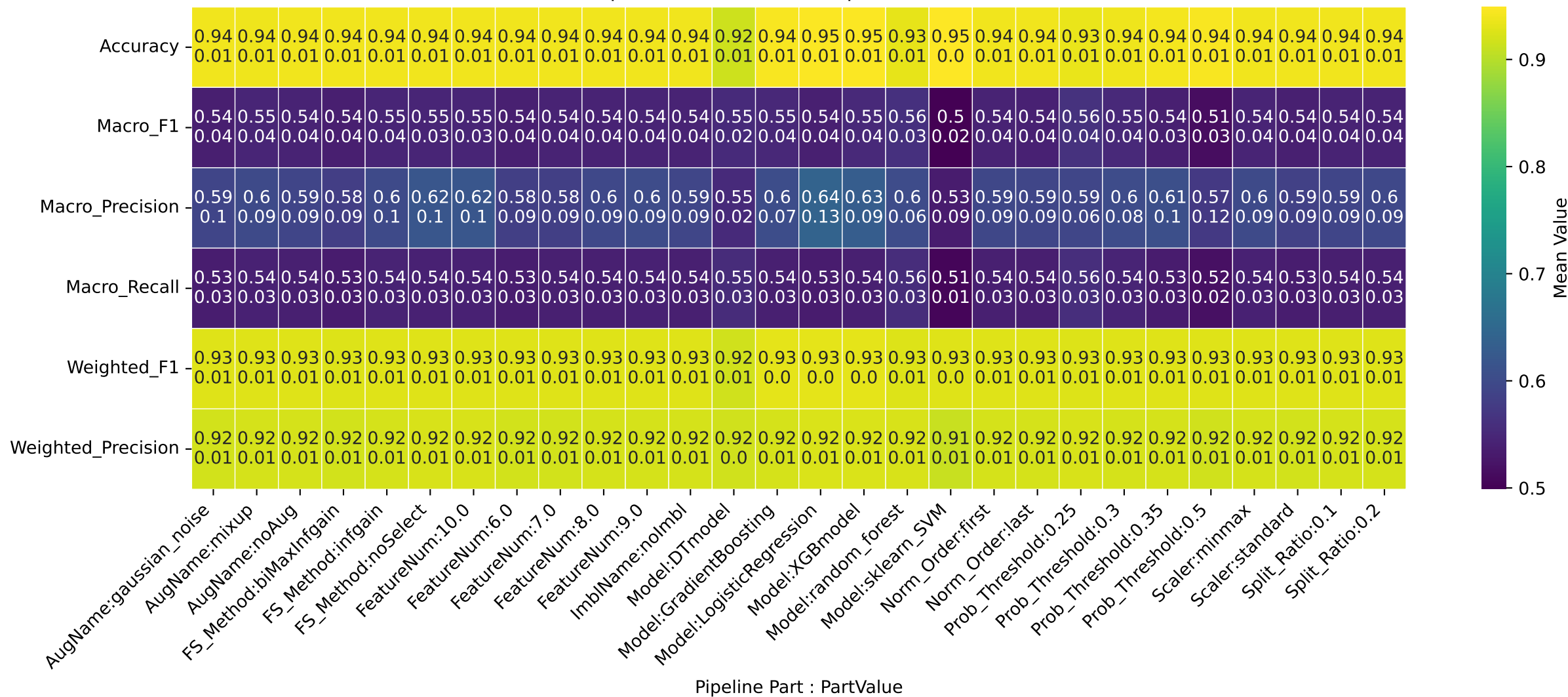
Pipeline Metrics Heatmap (Mean \pm Std)
