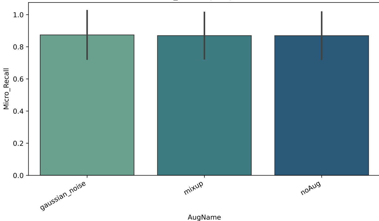
Micro_Recall by AugName
