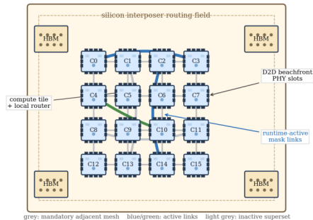
Top view: 2.5D chiplet NoI on silicon interposer
