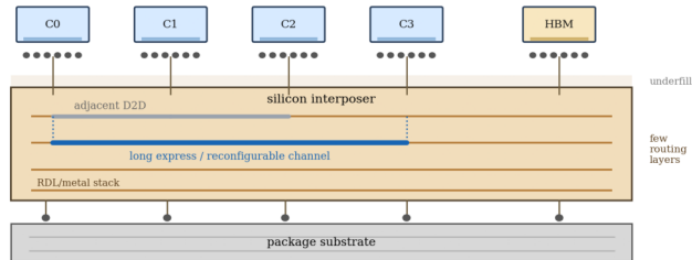
Side view: chiplets on a silicon interposer
