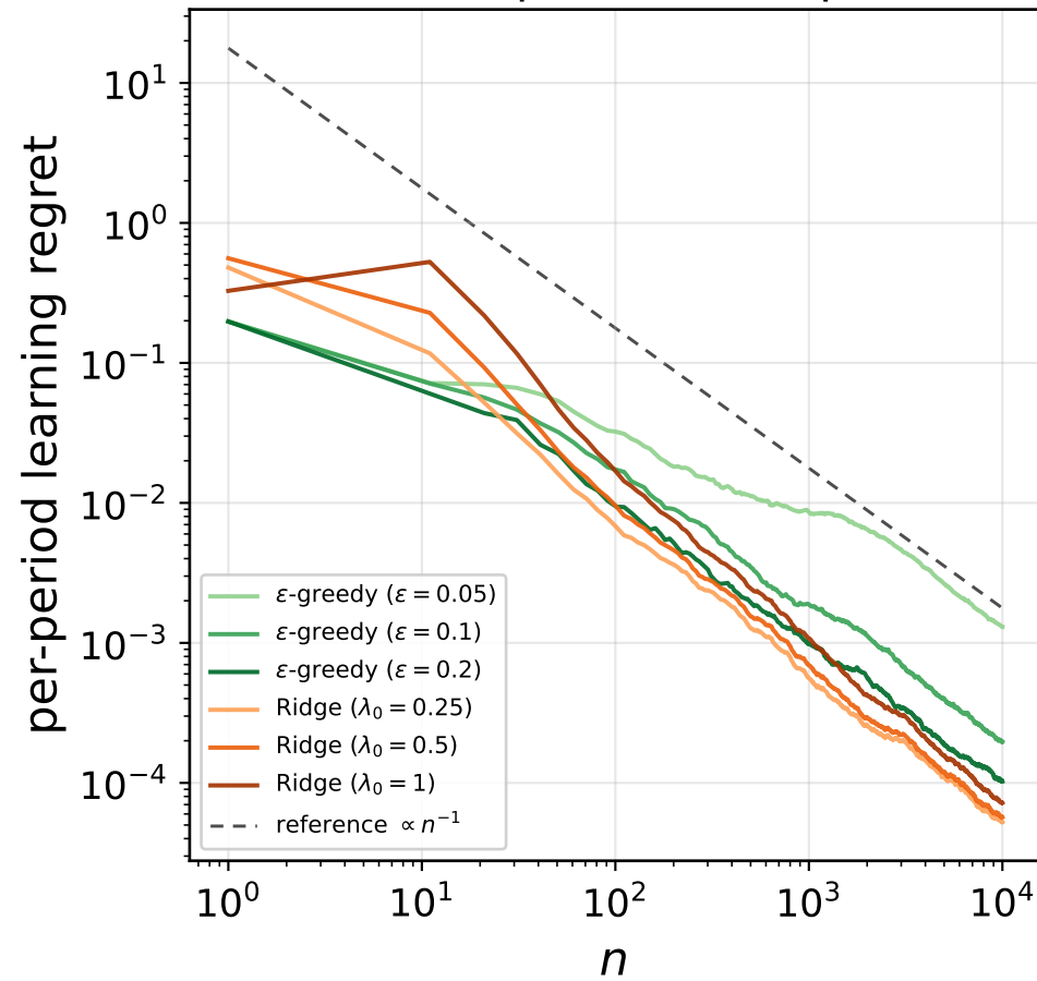
All-oblivious, persistent exploration
