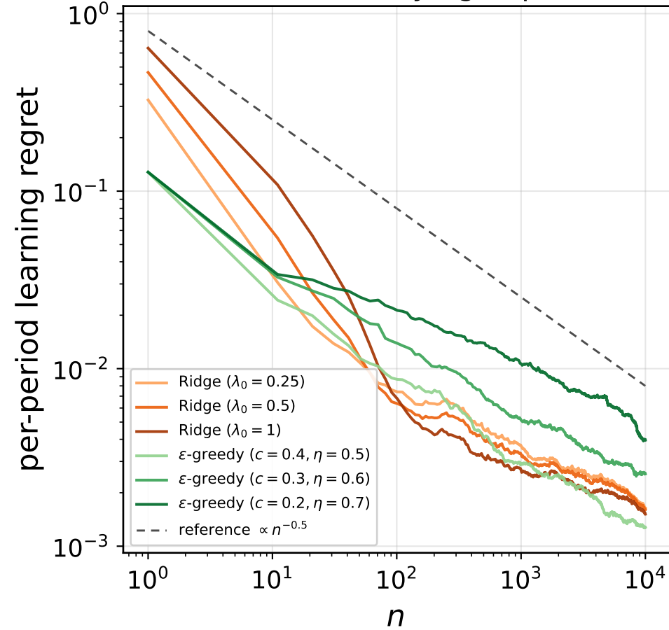
All-informed, decaying exploration
