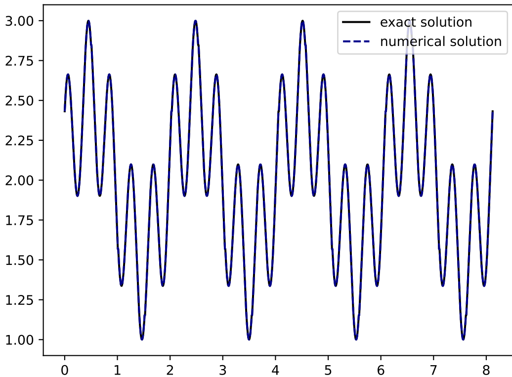
exact solution
