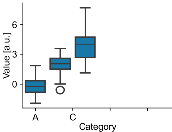
Group Distributions
