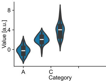
Distribution Shapes
