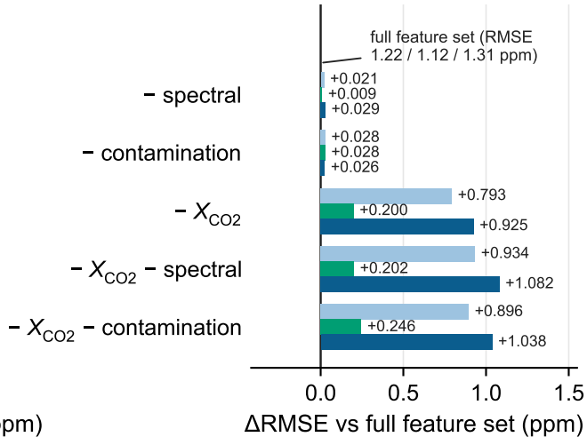
(b) deep-ensemble feature-set ablation
