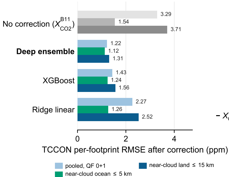
(a) baseline comparison
