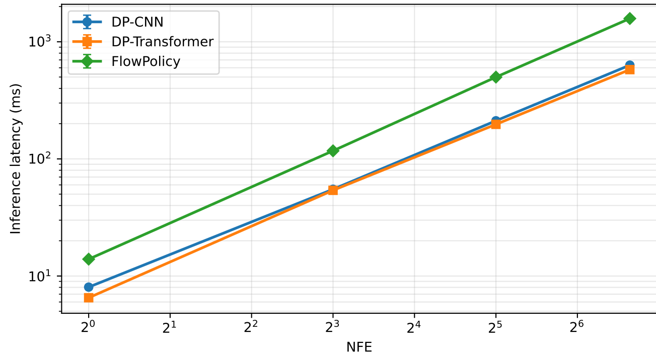
Latency vs NFE
