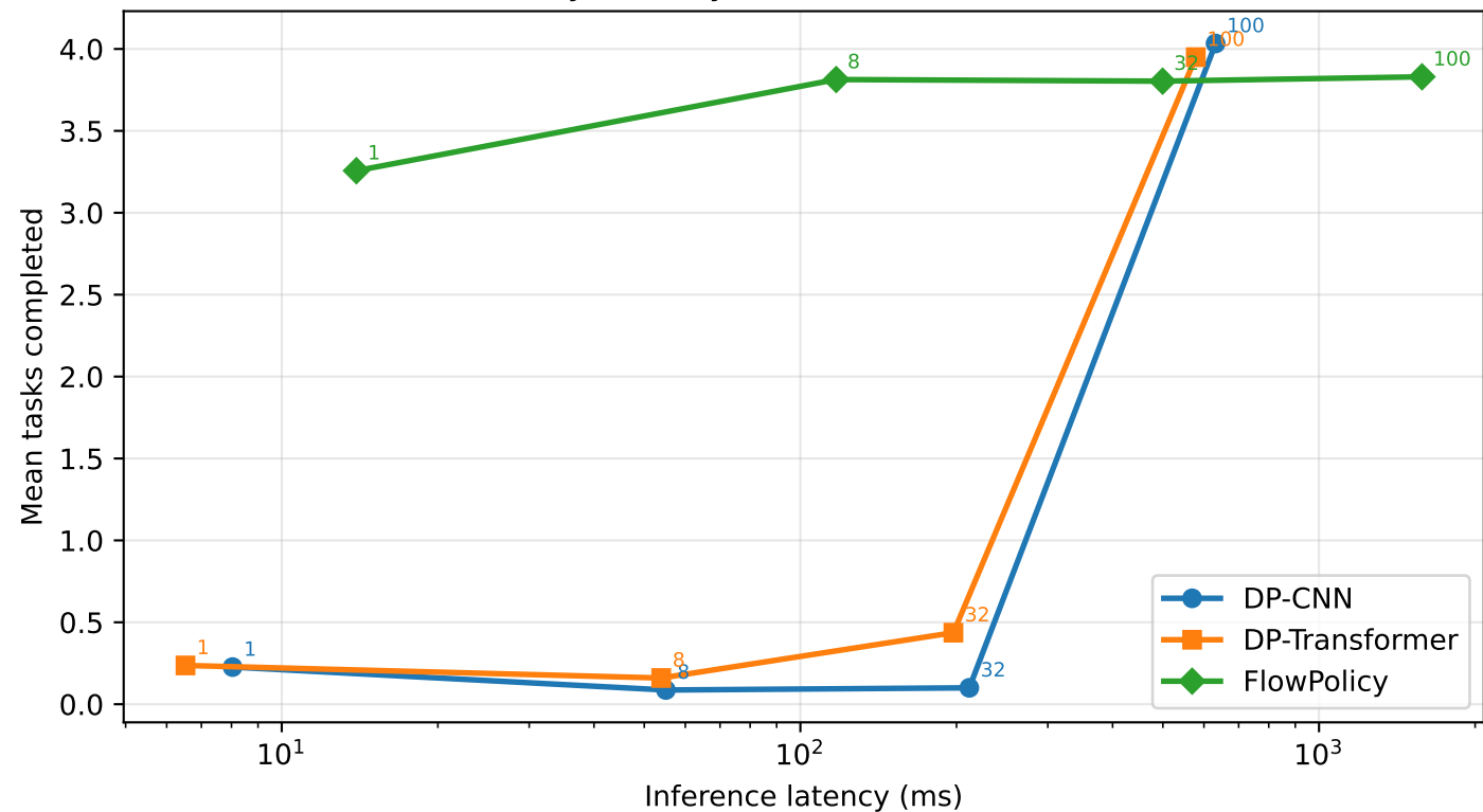
Quality-latency trade-off (labels = NFE)
