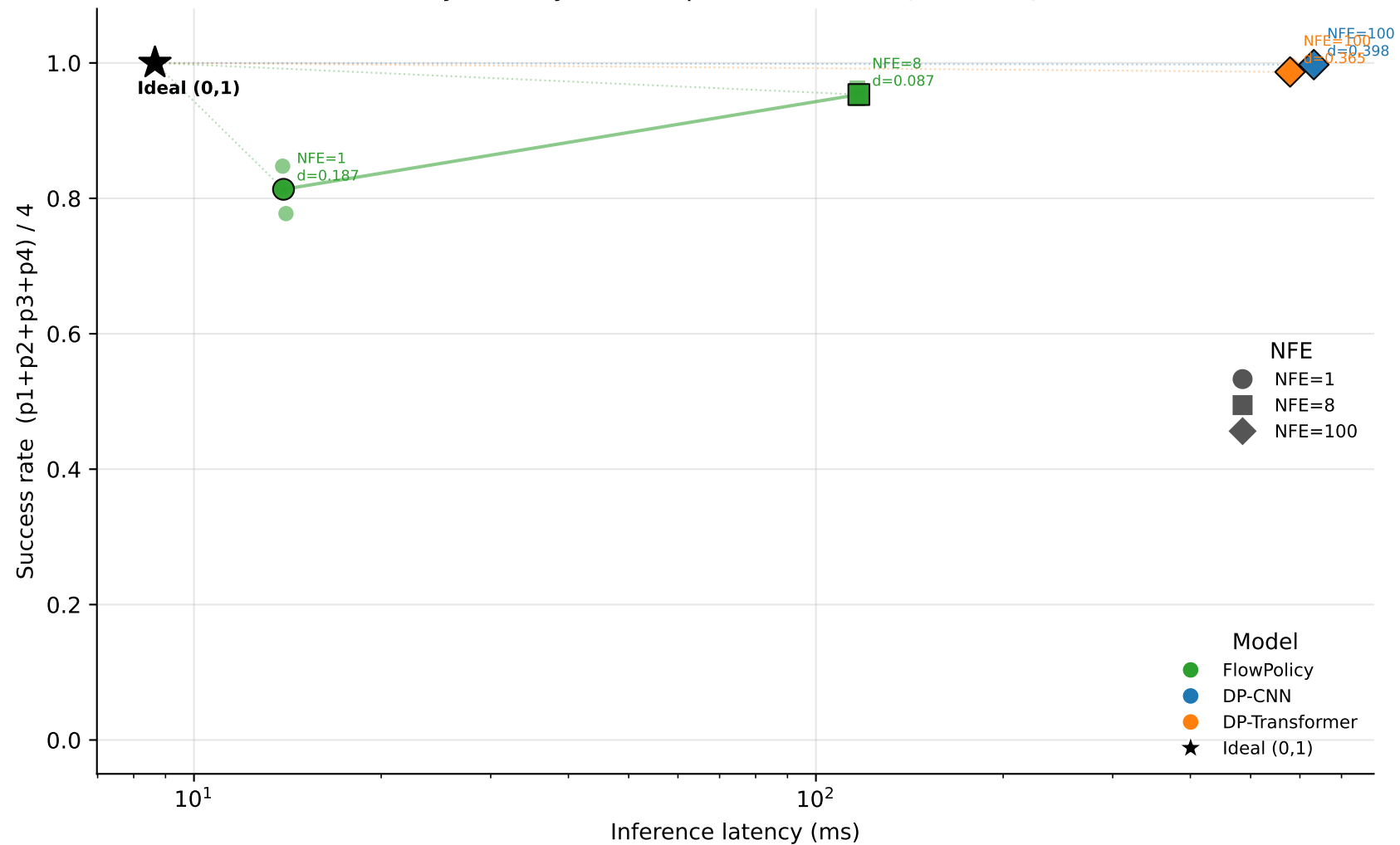
Quality-latency with utopia distance (FP@1/8, DP@100)
