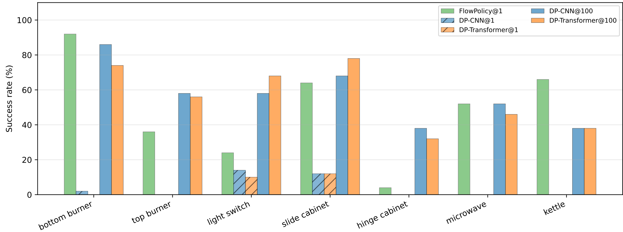
Per-task success: FlowPolicy@1 vs DP@1 (collapsed) vs DP@100
