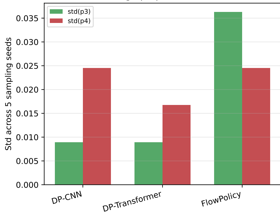
Multistage p3/p4 seed variance
