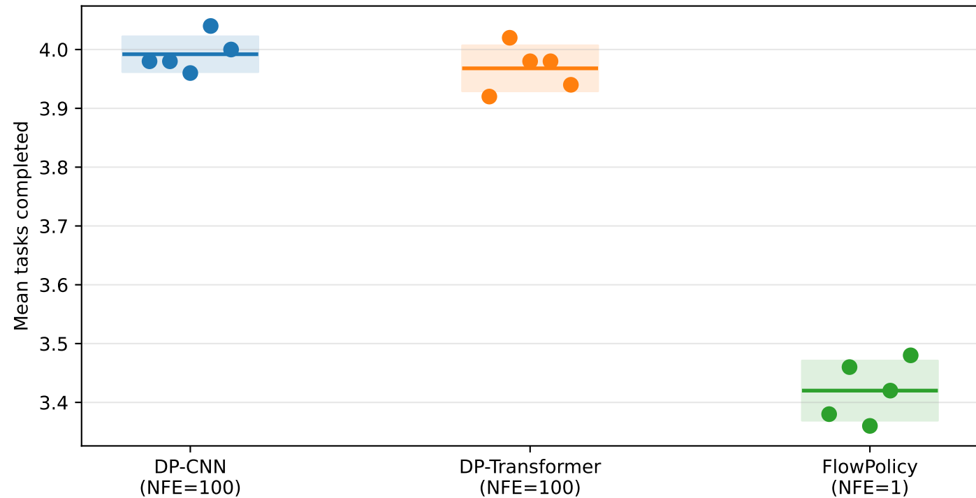
Per sampling-seed mean tasks (n=5) at default NFE
