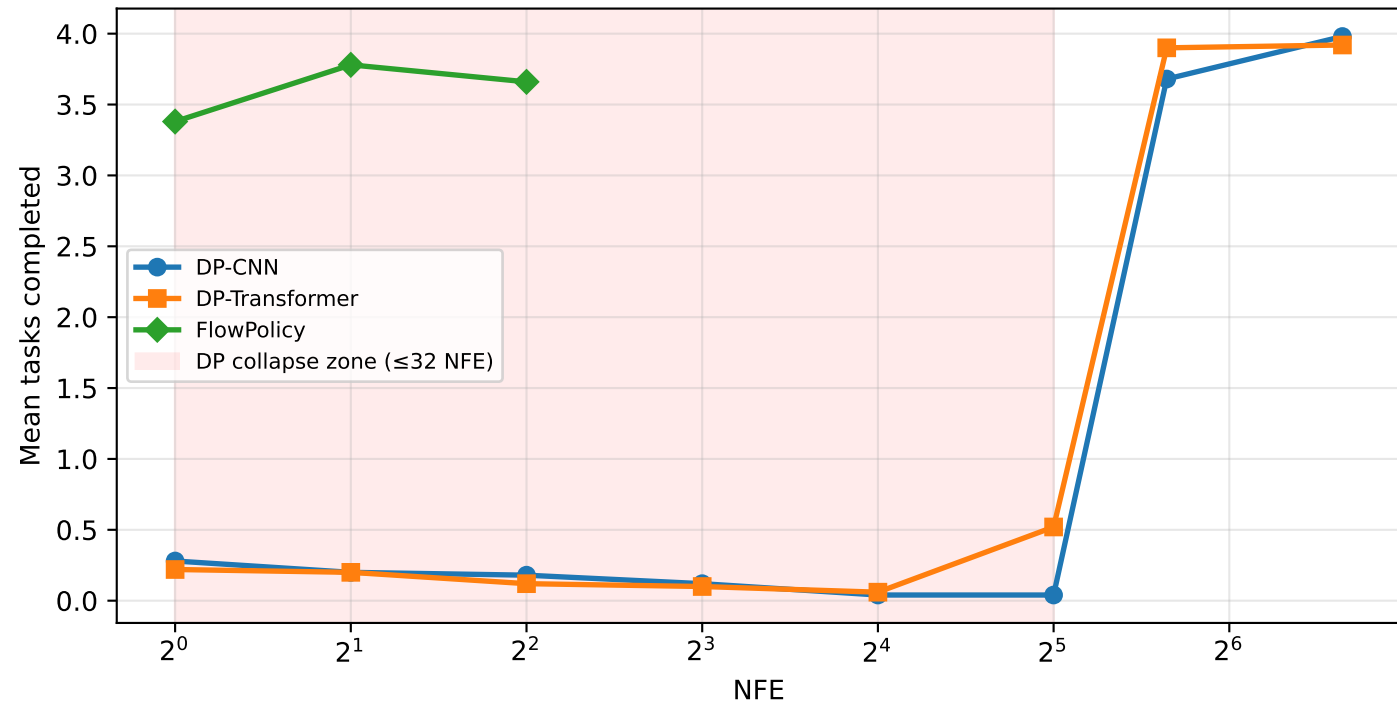
DP collapses below ~50 NFE; FlowPolicy stays usable at 1-4
