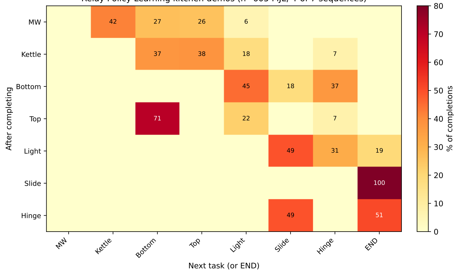
Demo dataset — P(\text{next} = B \mid \text{completed} = A) Relay Policy Learning kitchen demos (n=605 MJL, 4-of-7 sequences)
