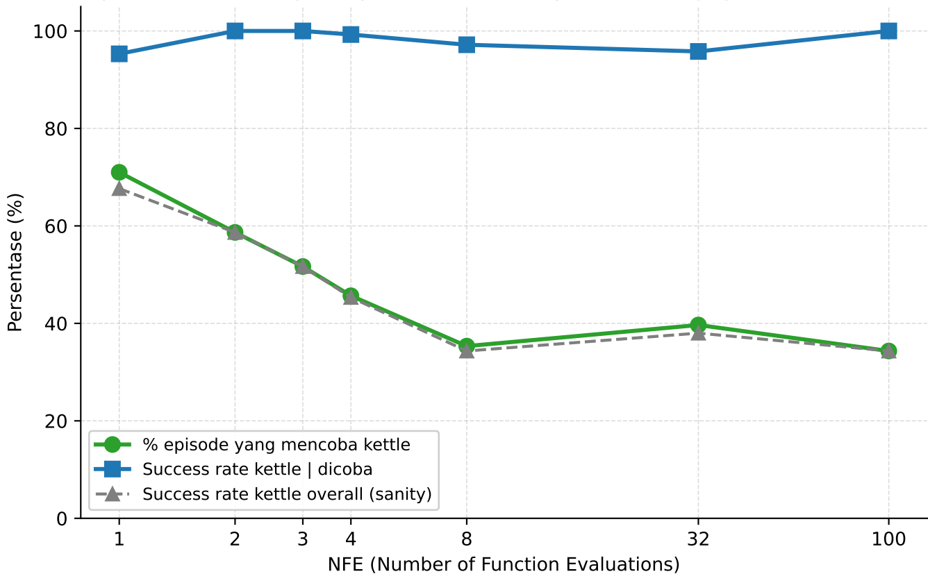
FlowPolicy kettle: attempt rate vs conditional success Drop overall SR mengikuti penurunan attempt, bukan kegagalan saat mencoba
