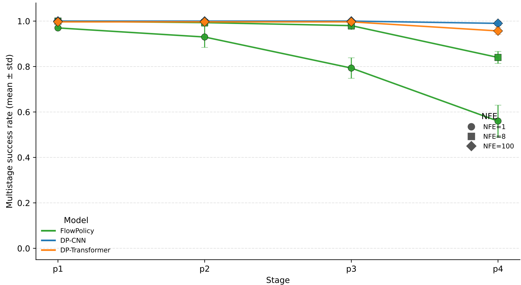
Multistage degradation p1→p4 (FP@1/8, DP@100) mean \pm std across 3 training seeds
