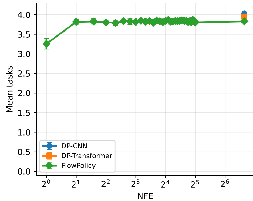
Mean tasks vs NFE
