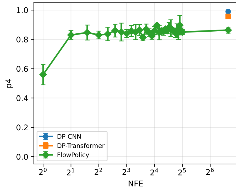
p4 vs NFE
