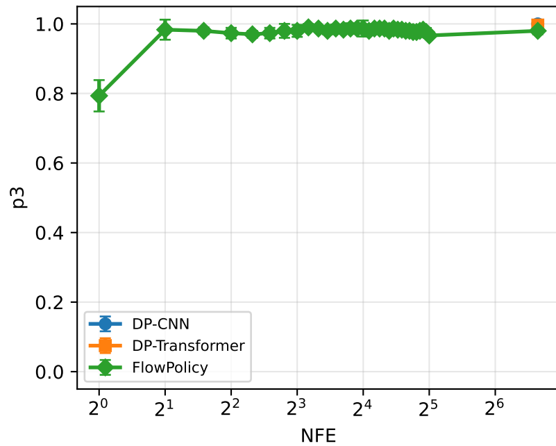
p3 vs NFE
