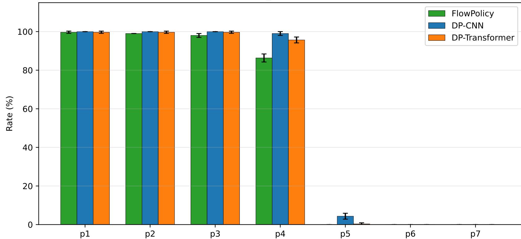
Multi-stage p_k (all @NFE=100)
