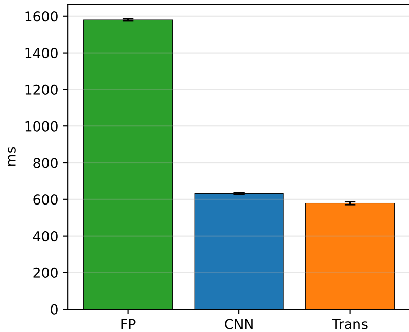
Inference latency
