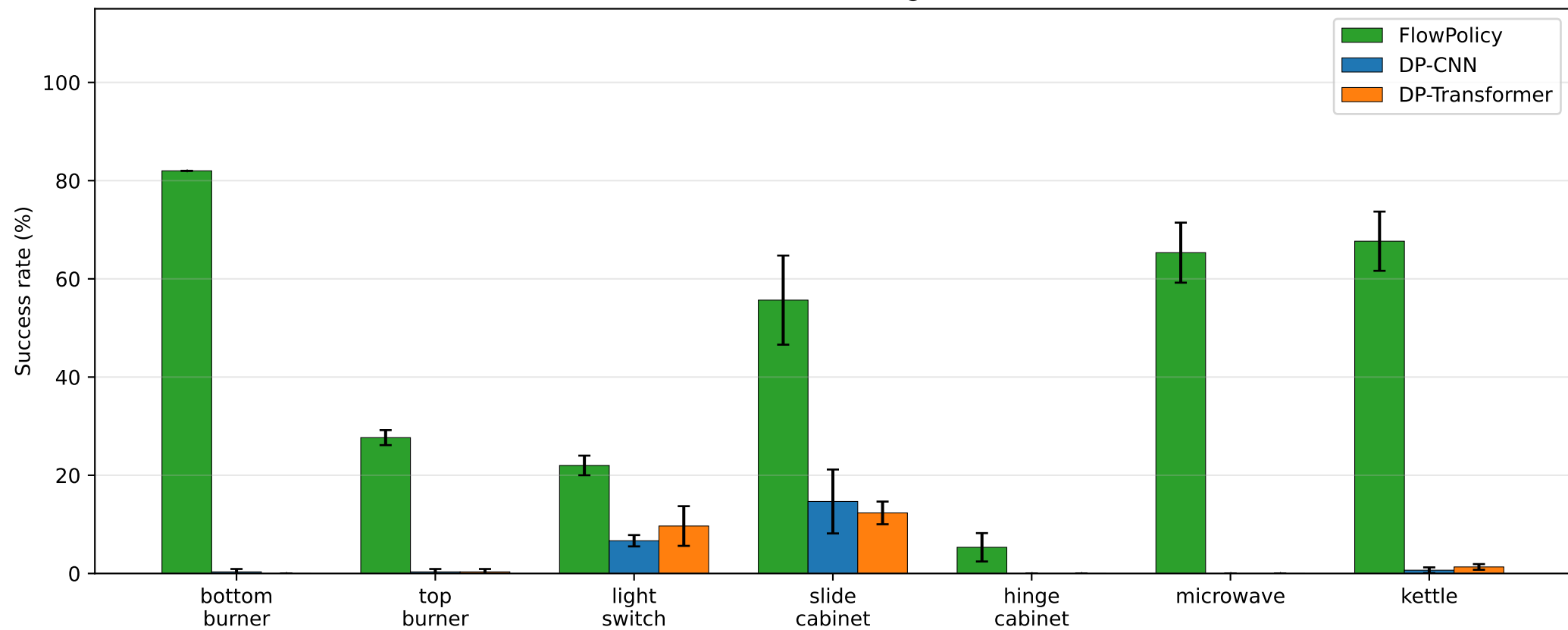
Per-task success (all @NFE=1)
