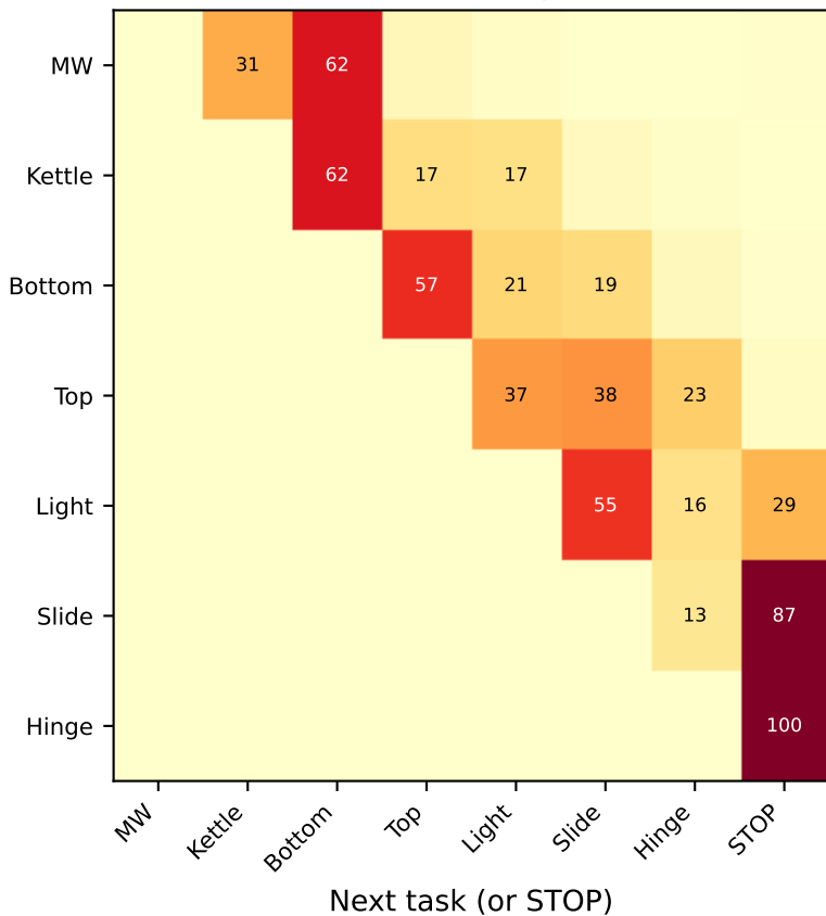
FlowPolicy
