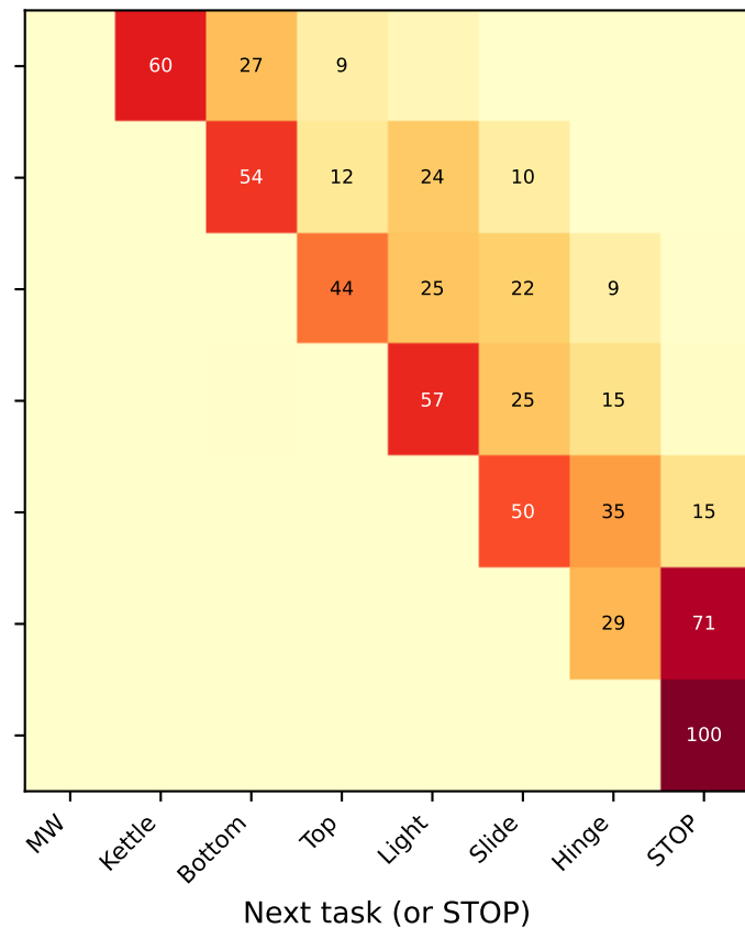
DP-Transformer
