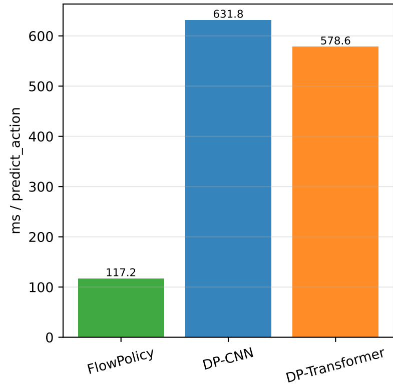
Inference latency
