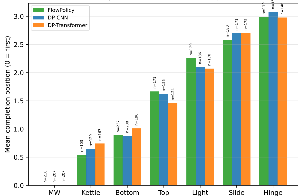
Mean position among completed episodes (lower = earlier in the chain)
