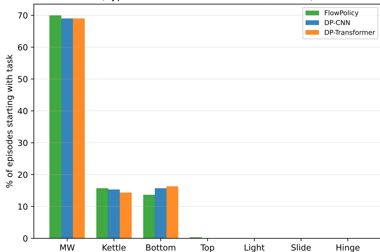
First completed task (hypothesis: FP starts with kettle/bottom?)
