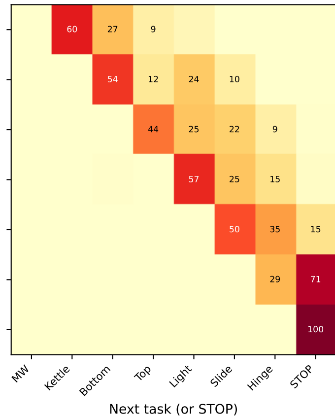
DP-Transformer @ NFE=100
