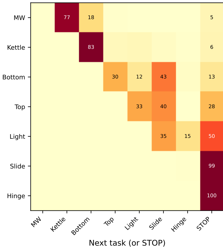
FlowPolicy @ NFE=1
