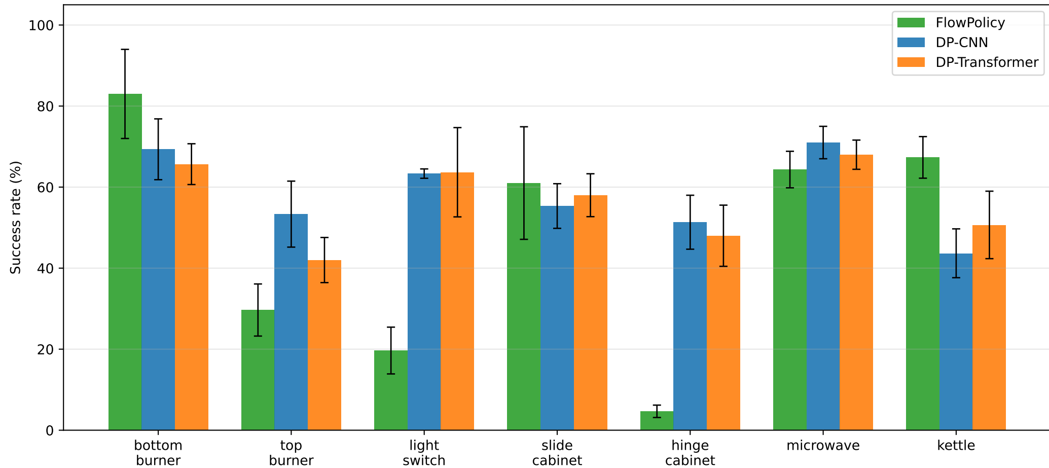
Per-task success rate (mean \pm std across 3 seeds) Denominator: n=300 episodes per model (fair comparison)
