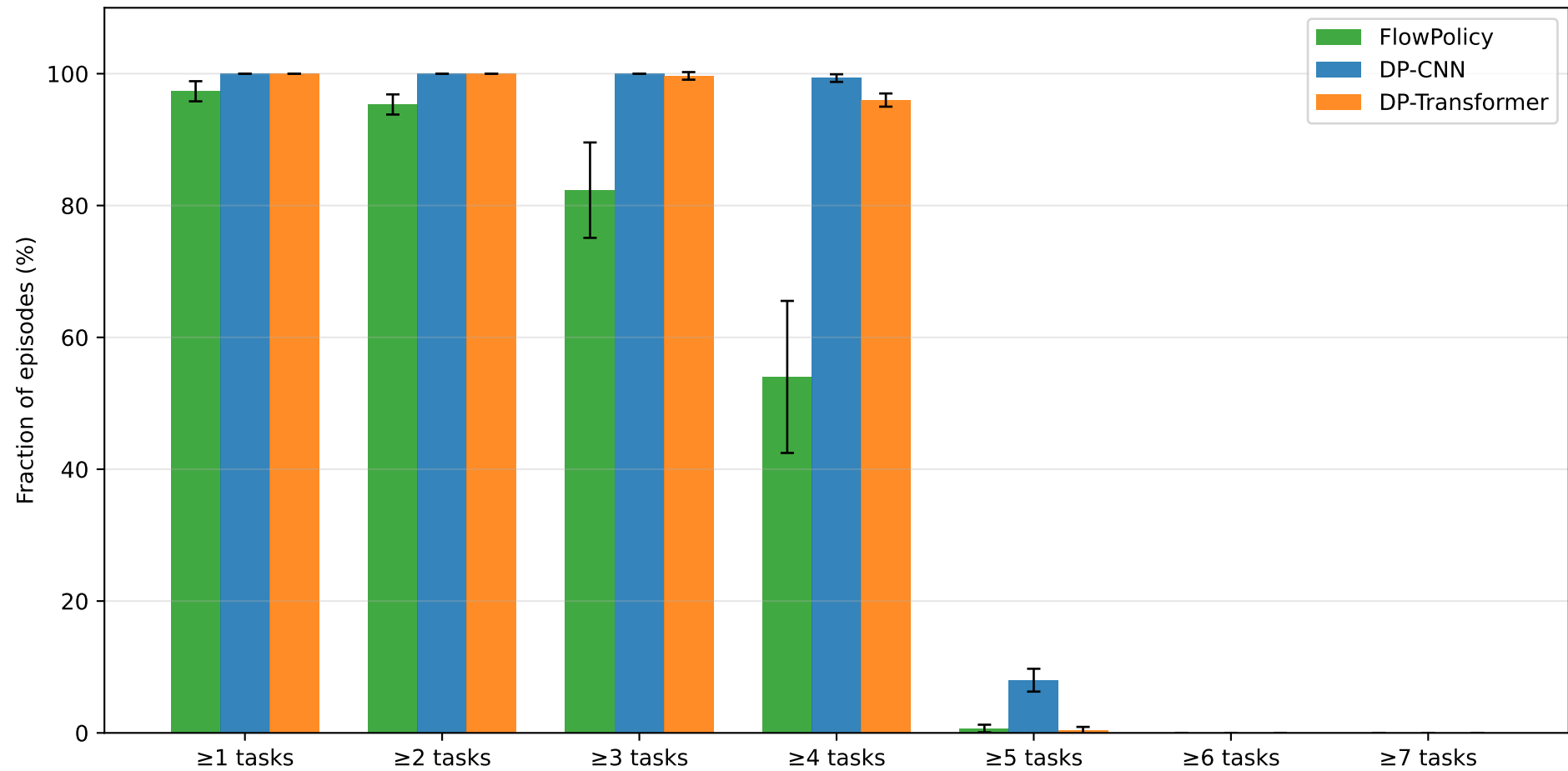
Multi-stage p_k: fraction of episodes completing \geq k of 7 tasks n=300 episodes per model
