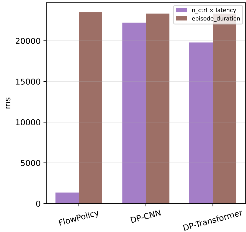
Inference budget vs wall-clock episode
