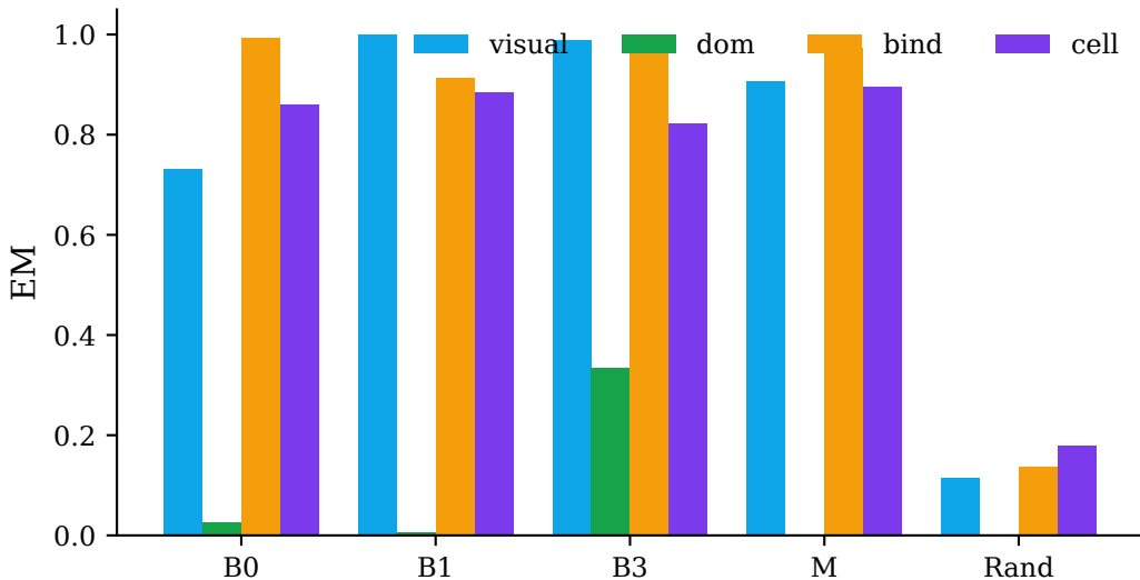
Hard-struct probes
